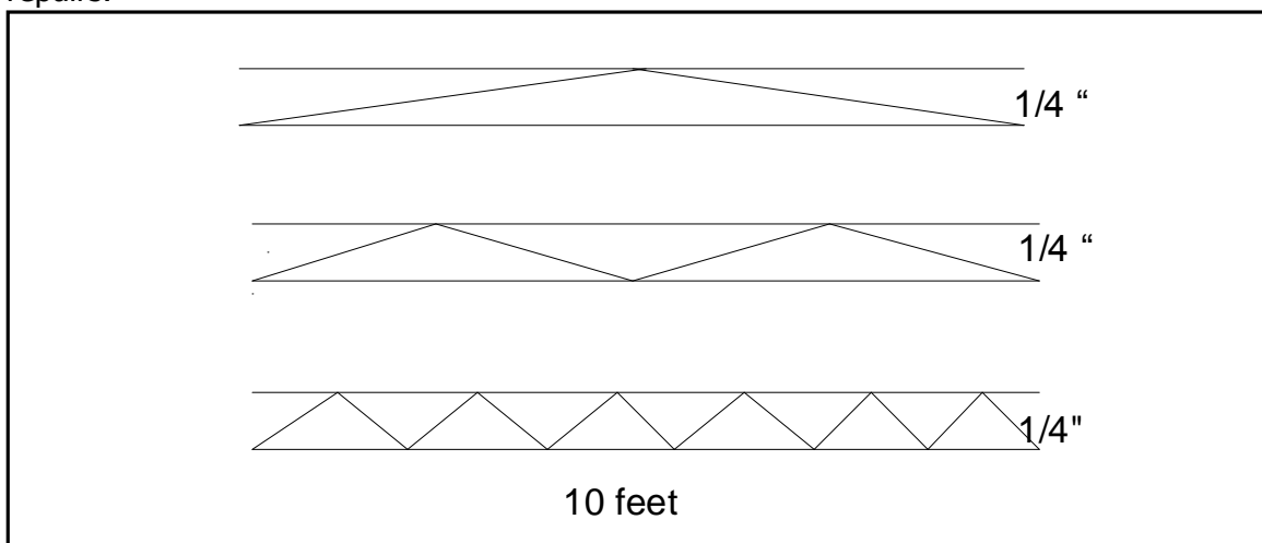
Figure 1 - All three profiles comply with the same acceptable tolerance 1/4 in. (6 mm) in 10 ft. (3 m) using the straightedge method (diagram is not to scale and exaggerated for clarity)
